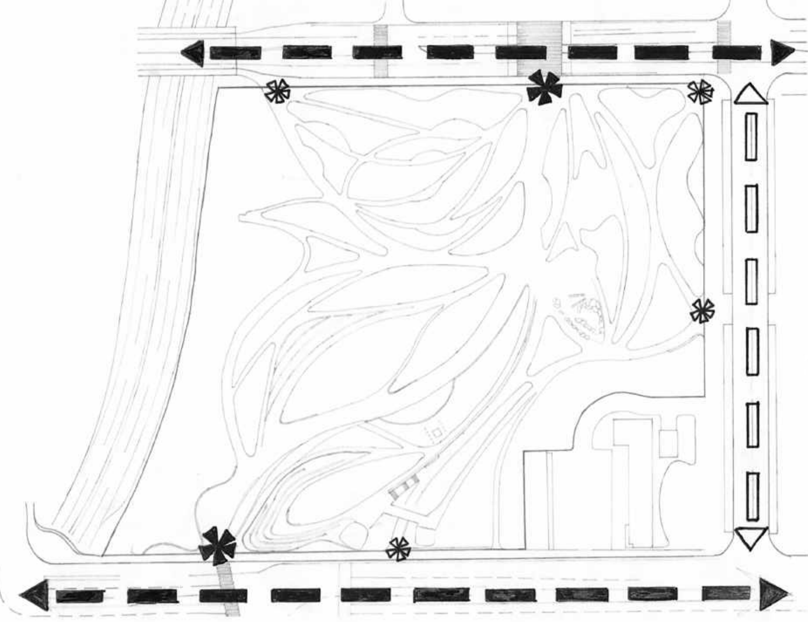
VEHICULAR CIRCULATION + ACCESS POINTS
