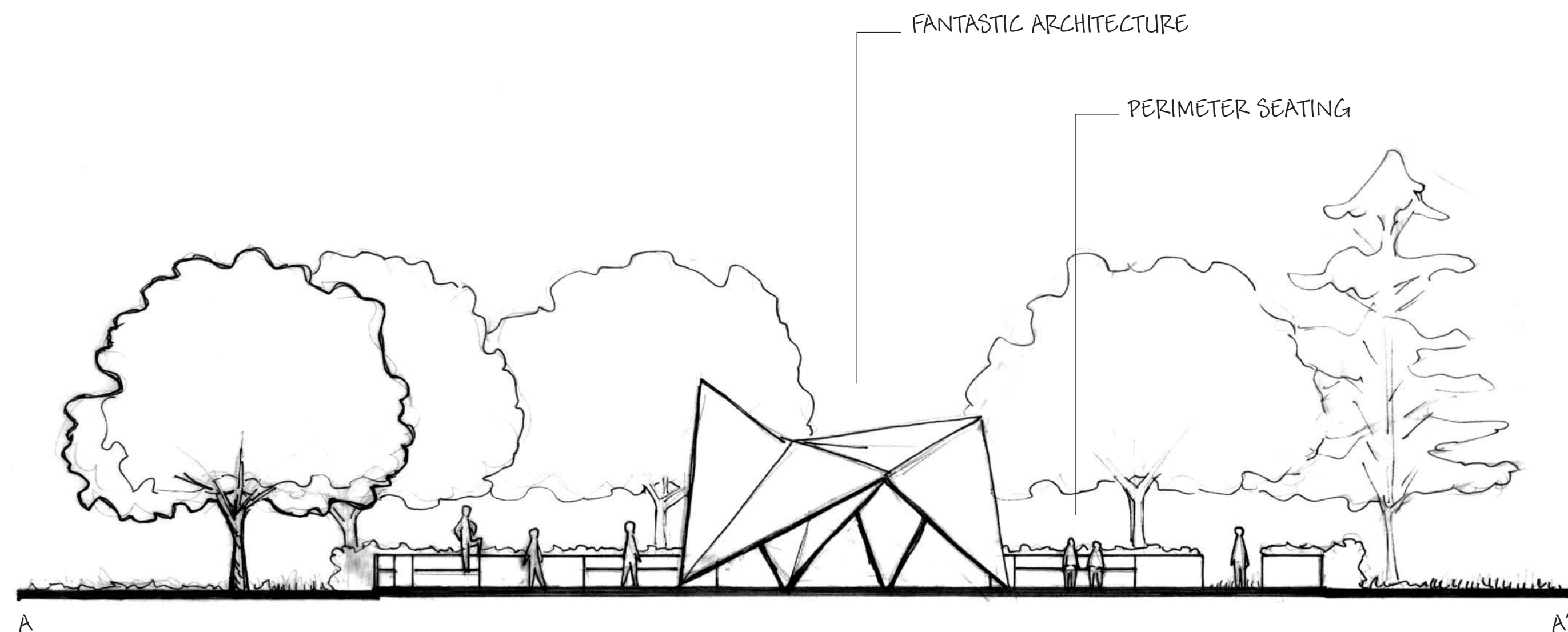
SECTION-ELEVATION A-A'
