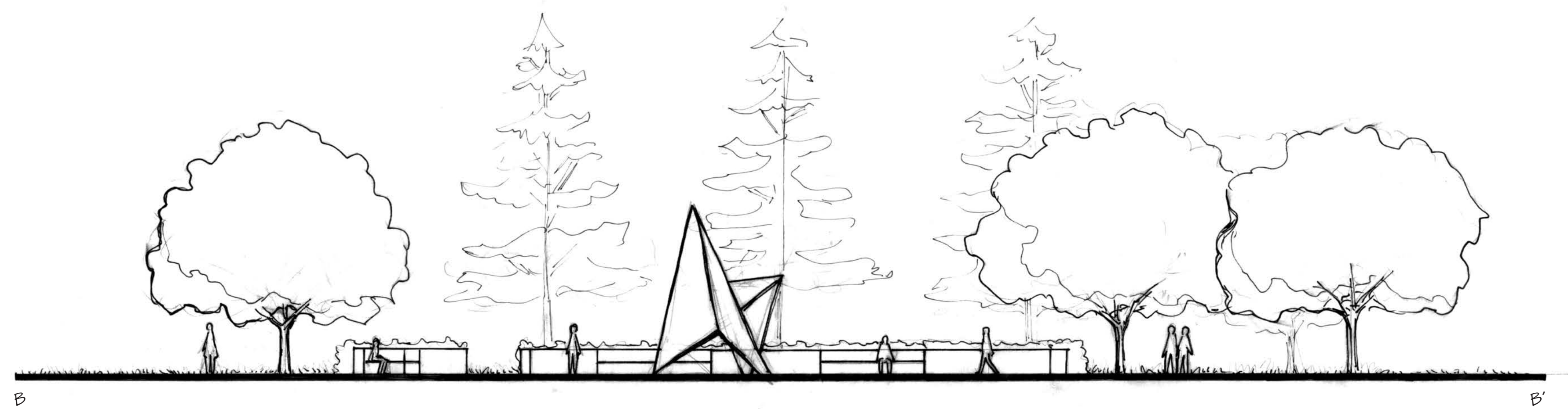
SECTION-ELEVATION B-B'
